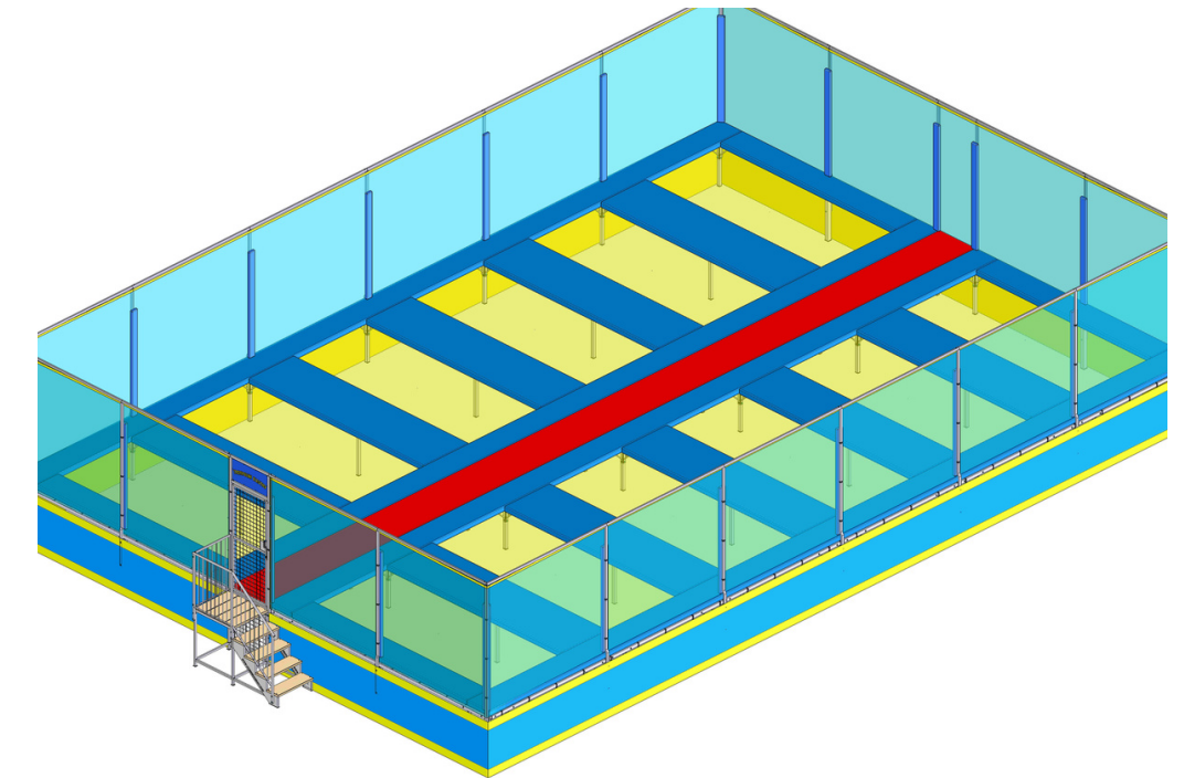
ART. 112.1 - Trampoline 12 standard seats in two lines, central corridor
