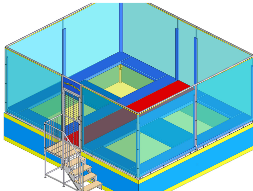
ART. 104.3 - Trampoline 4 mini seats in line, lateral corridor
